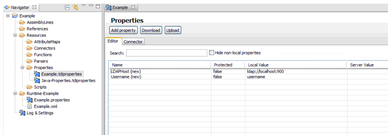
Figure 8. Properties view
