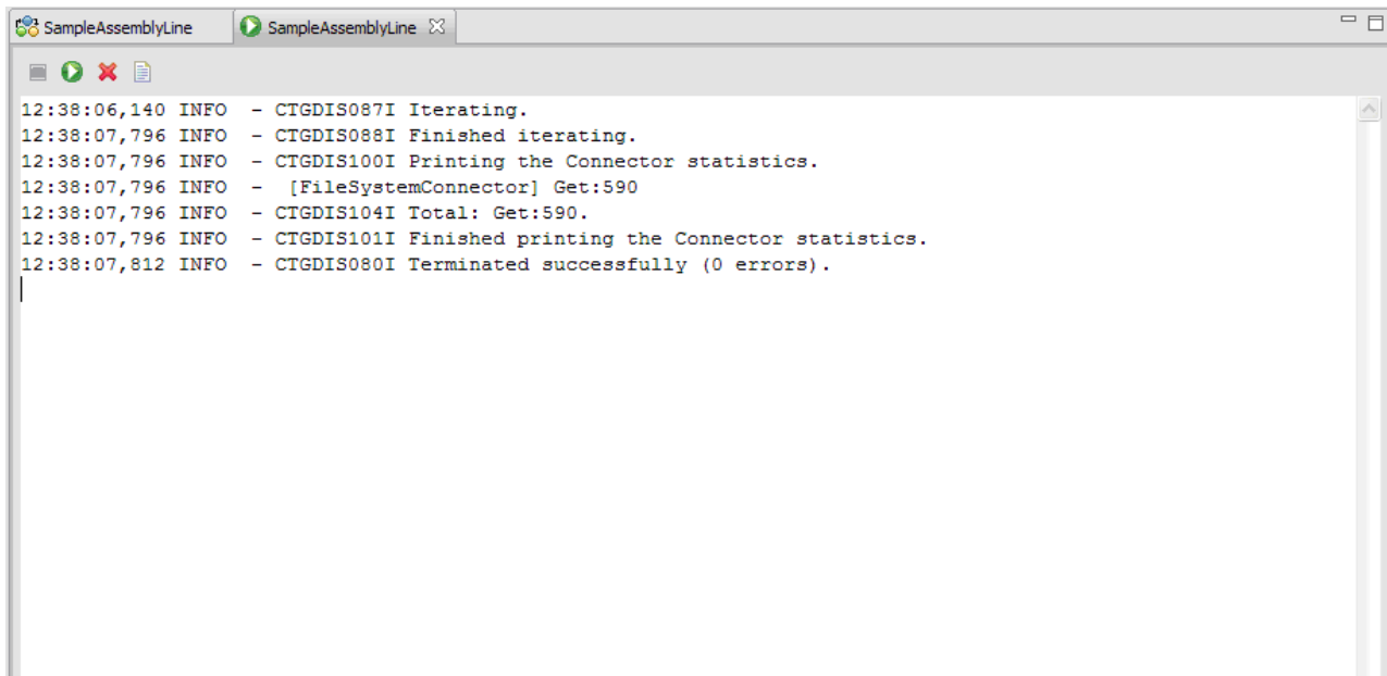
Figure 29. Console log
