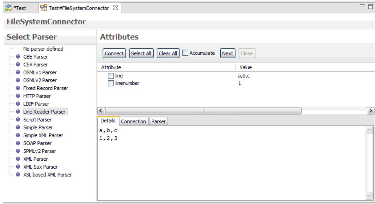
Figure 48. Stream Data Browser
