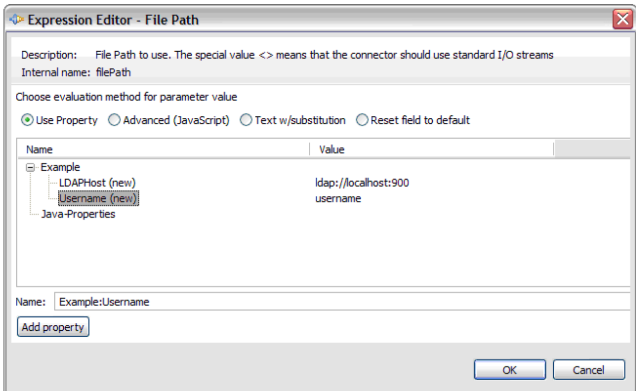
Figure 40. Expression Editor window, simple mode
