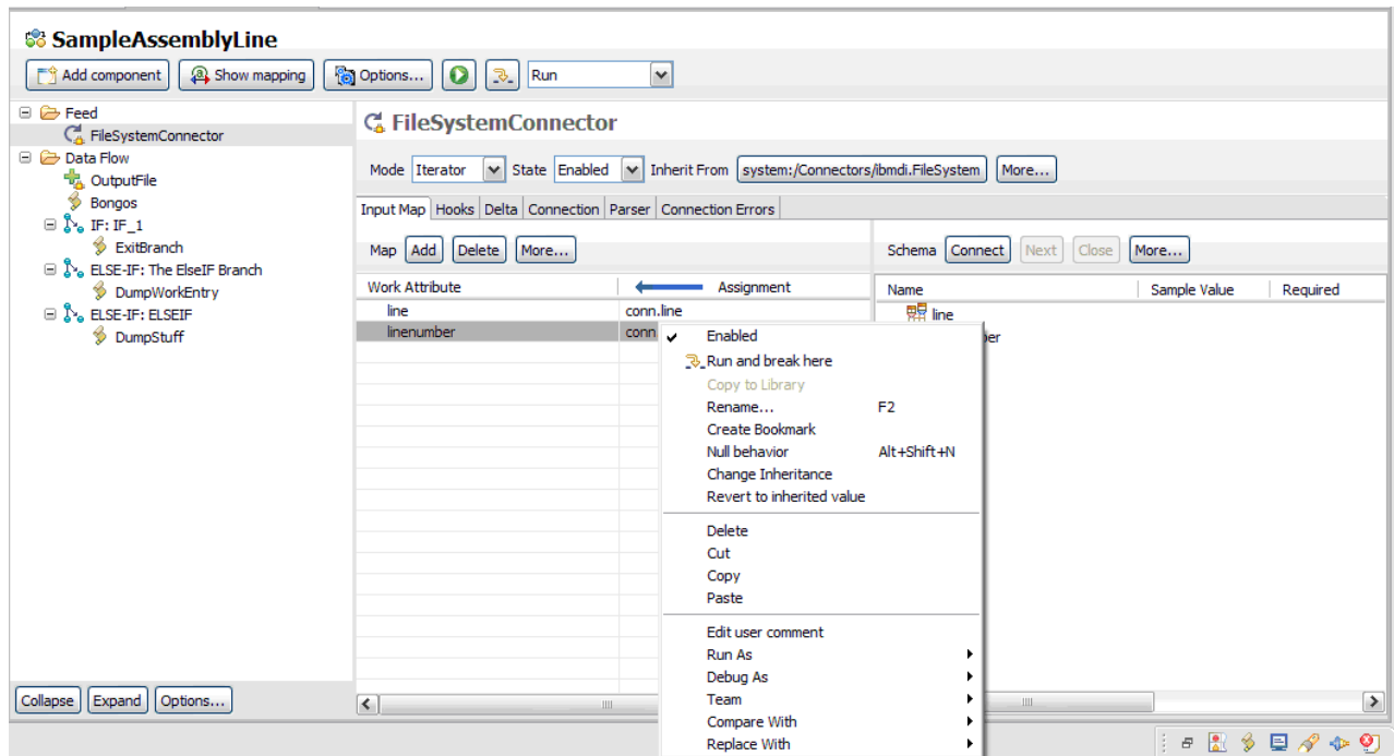
Figure 32. Attribute Mapping, with discovered Attributes
