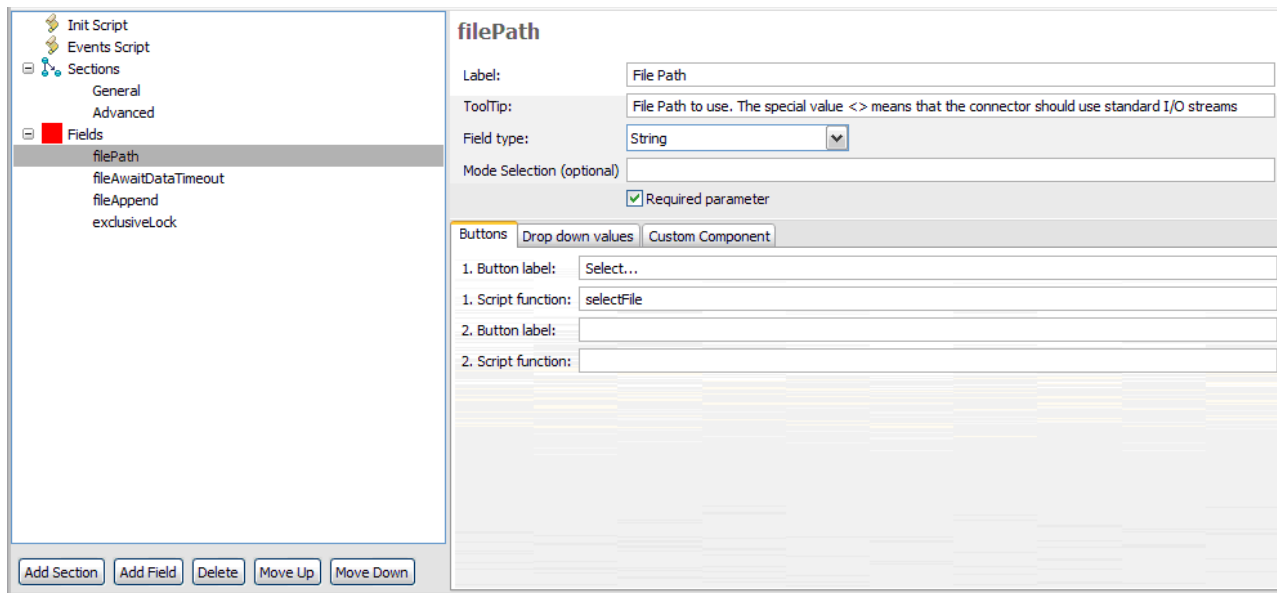
Figure 61. Forms Editor - field definitions
