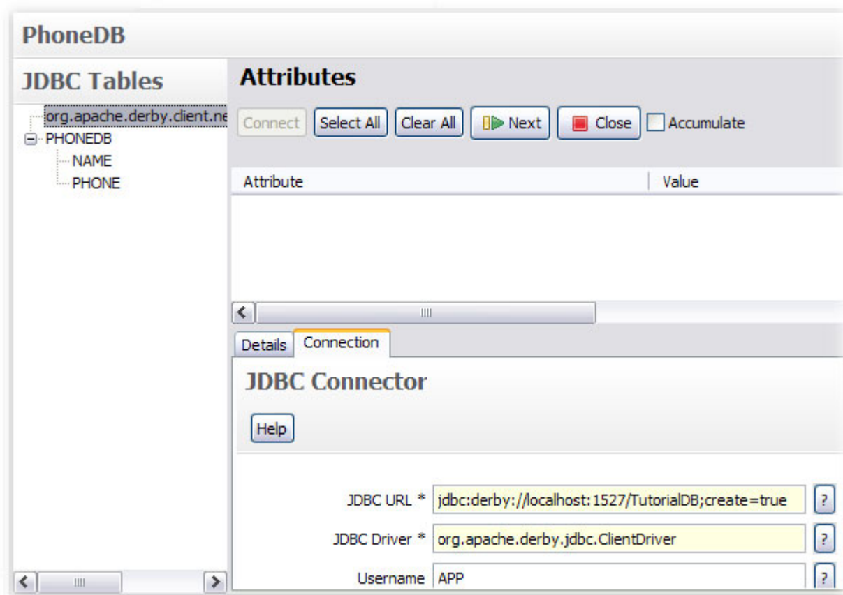
Figure 49. JDBC Data Browser
