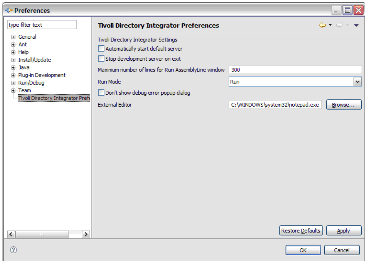
Figure 80. Configuration Editor Preferences window
