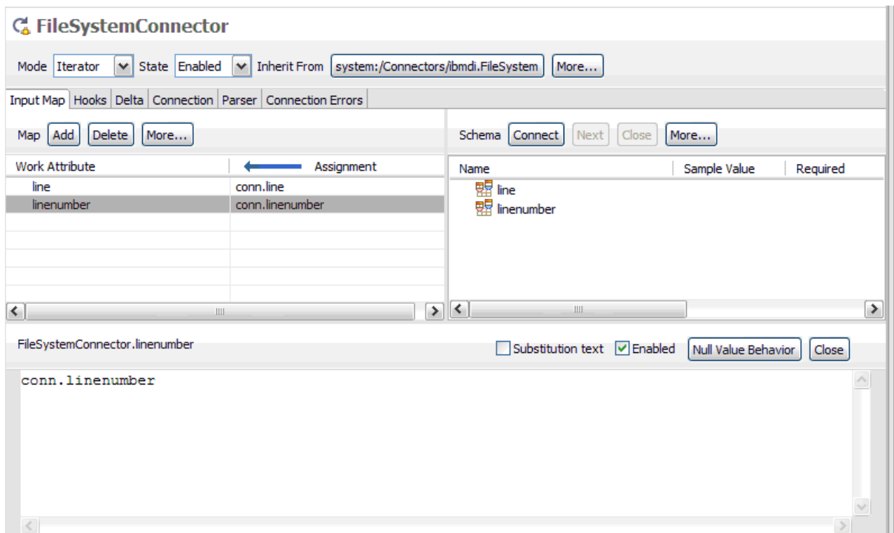
Figure 34. Attribute Mapping, with JavaScript editing window for individual Attribute
