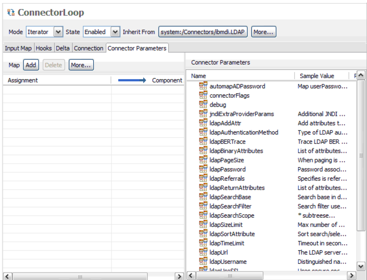
Figure 27. Connector Parameters in Connector Loop
