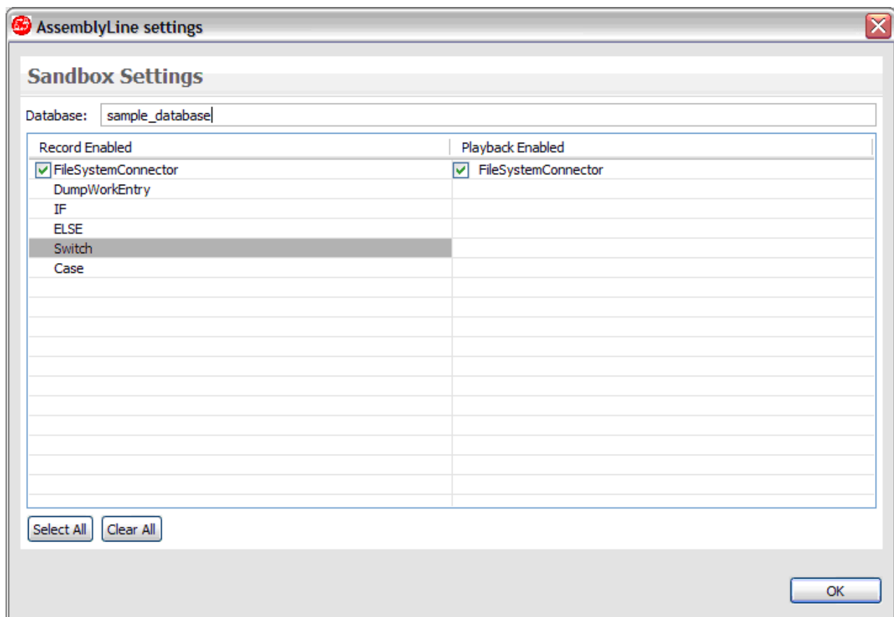
Figure 21. AssemblyLine Sandbox settings
