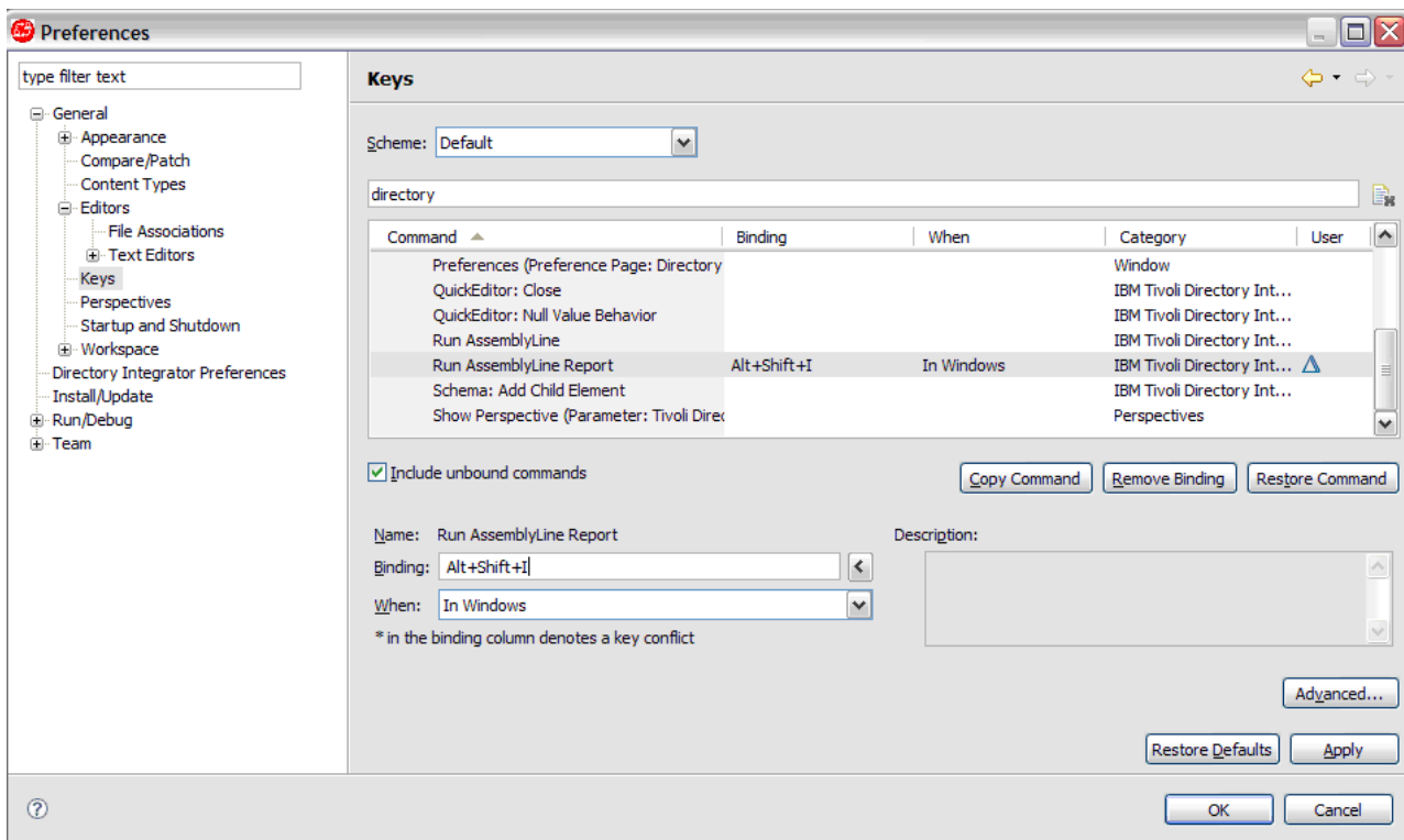
Figure 88. Key Assignments window
