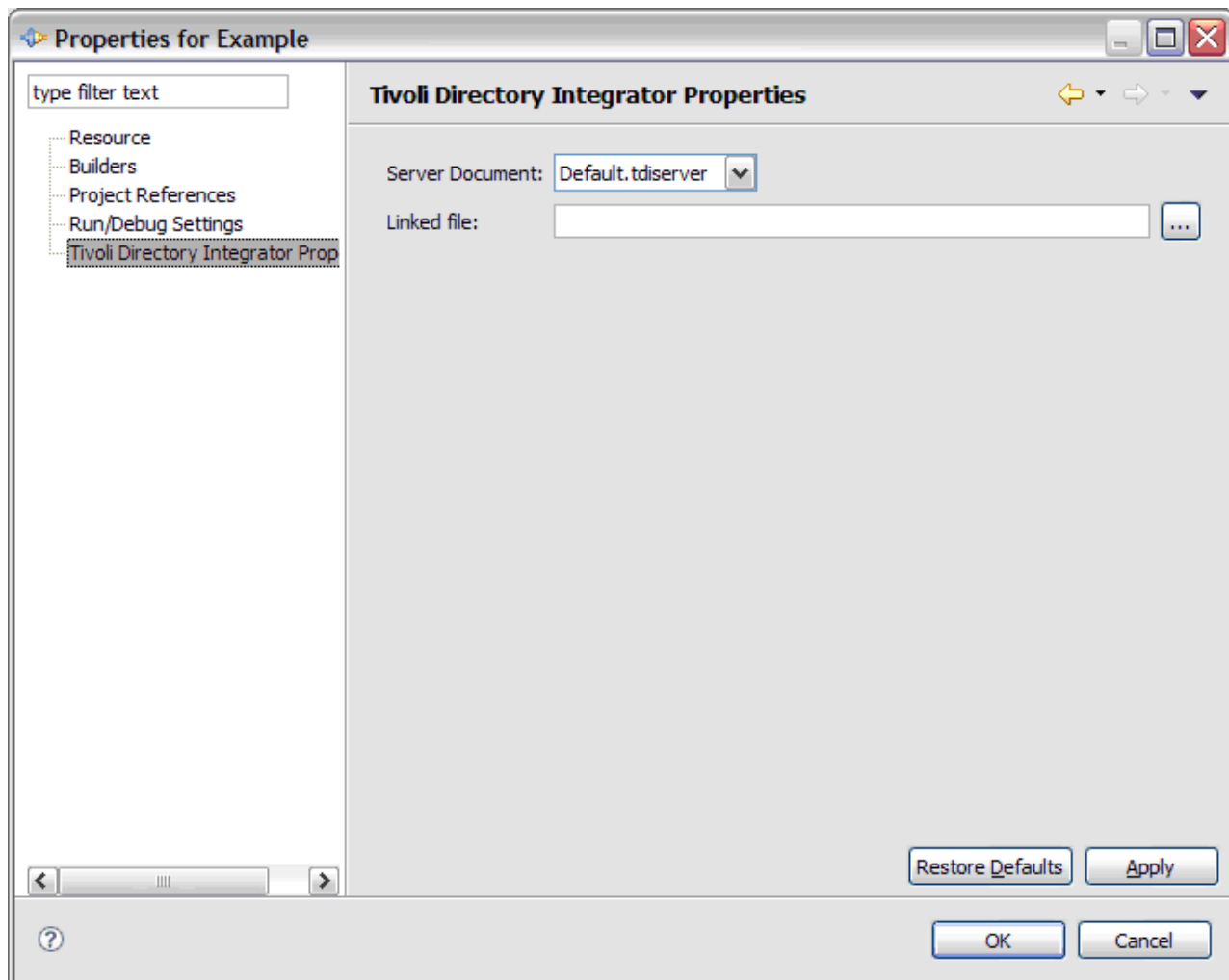
Figure 77. Project Properties
