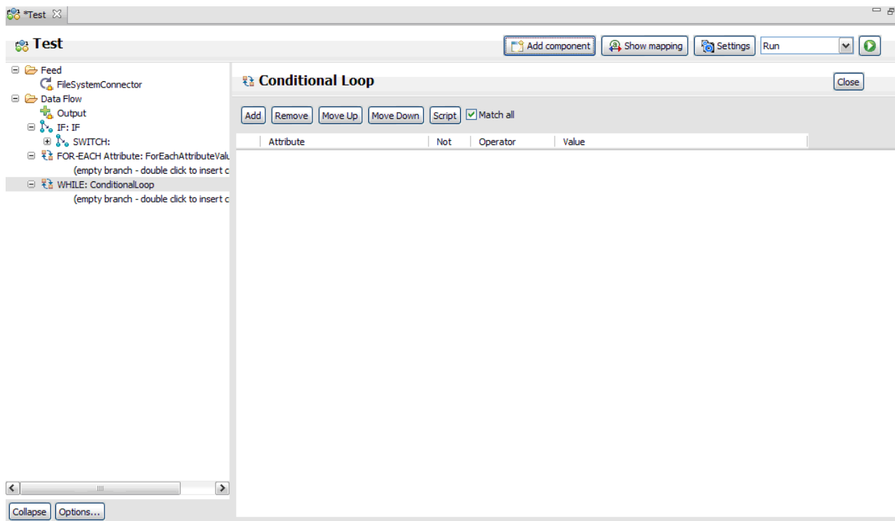
Figure 25. Conditional loop
