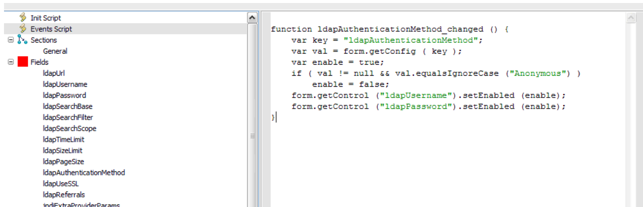
Figure 58. Forms Editor, Events Script in LDAP Connector
