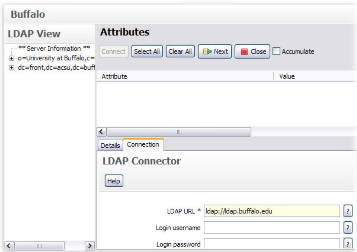
Figure 52. LDAP Data Browser
