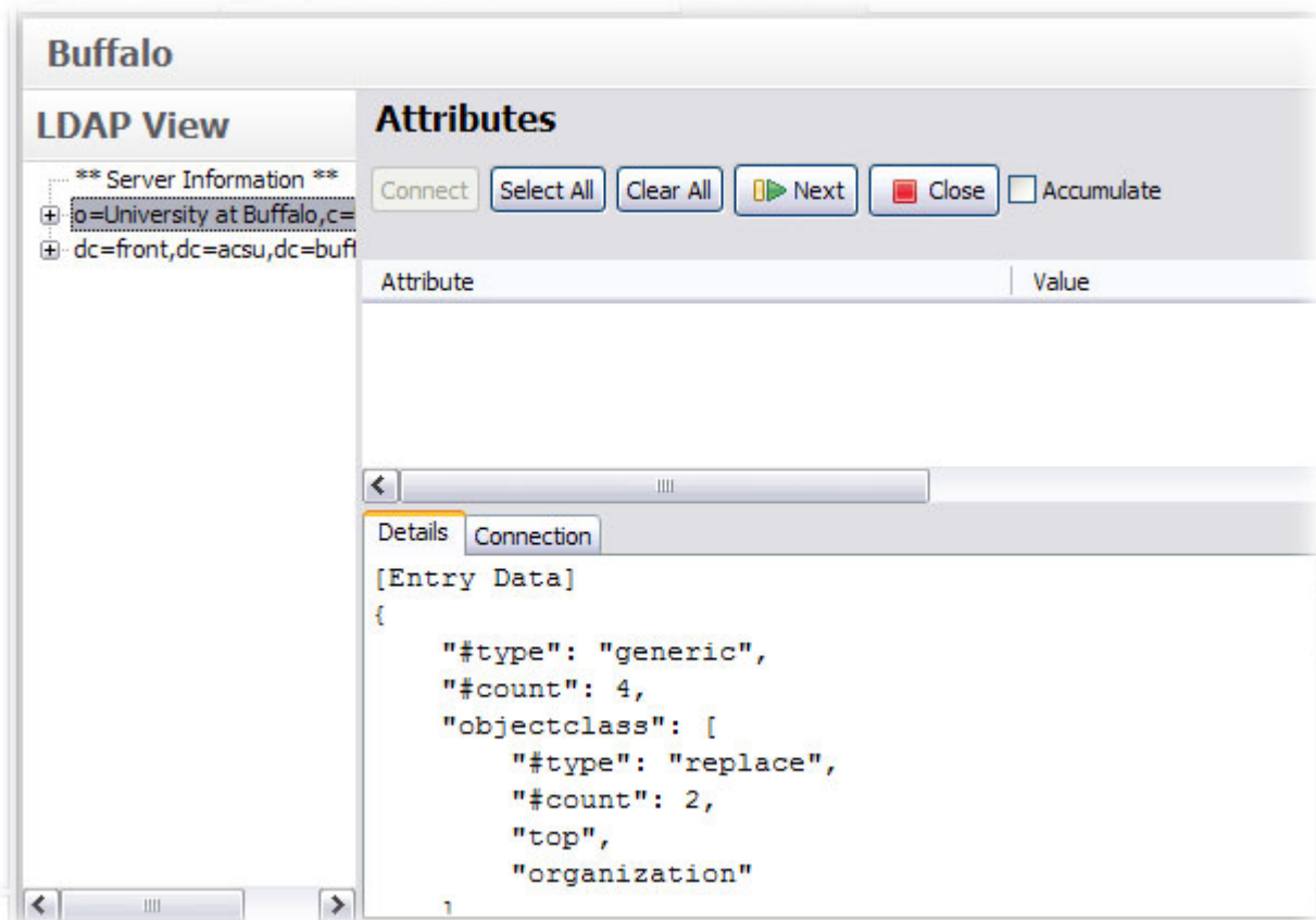
Figure 53. LDAP Data Browser entry
