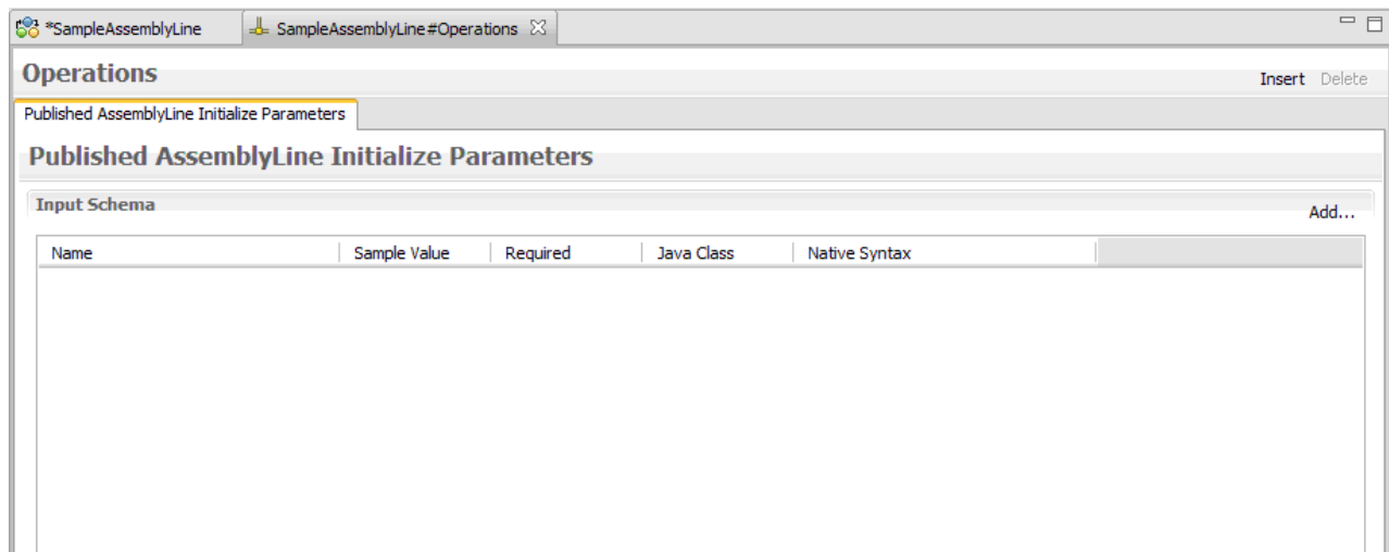
Figure 18. AssemblyLine Operations
