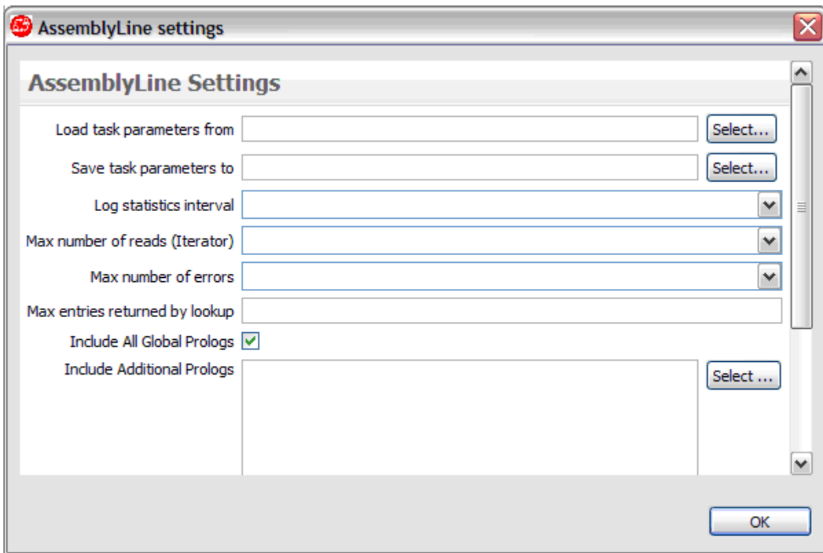
Figure 15. AssemblyLine Settings
