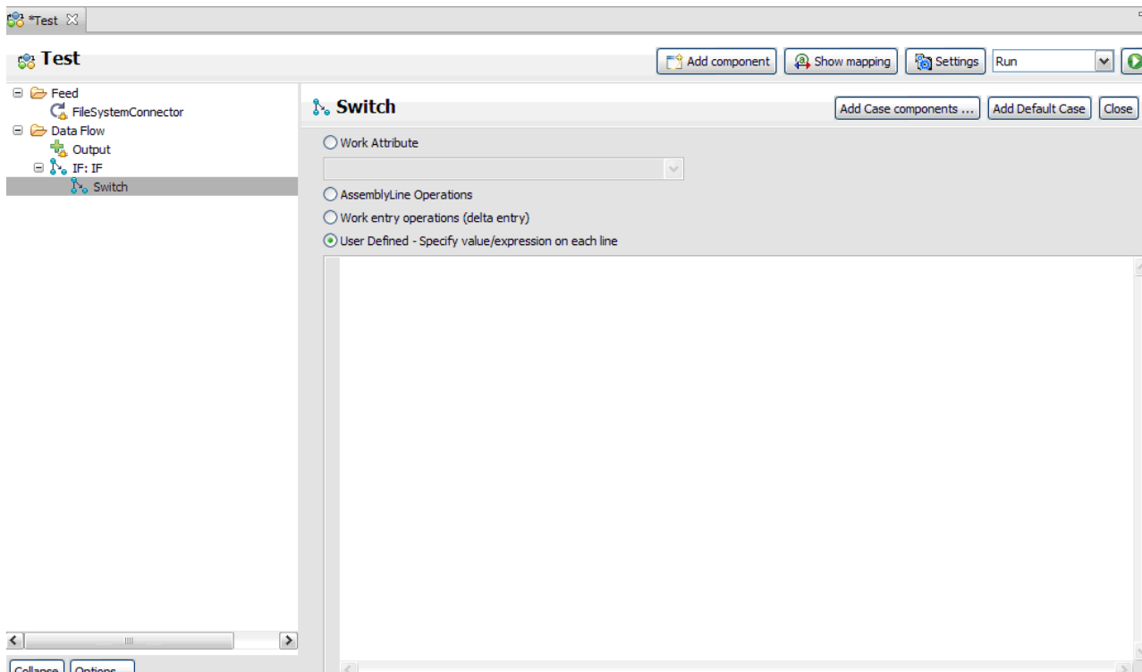
Figure 23. Switch/Case Branch
