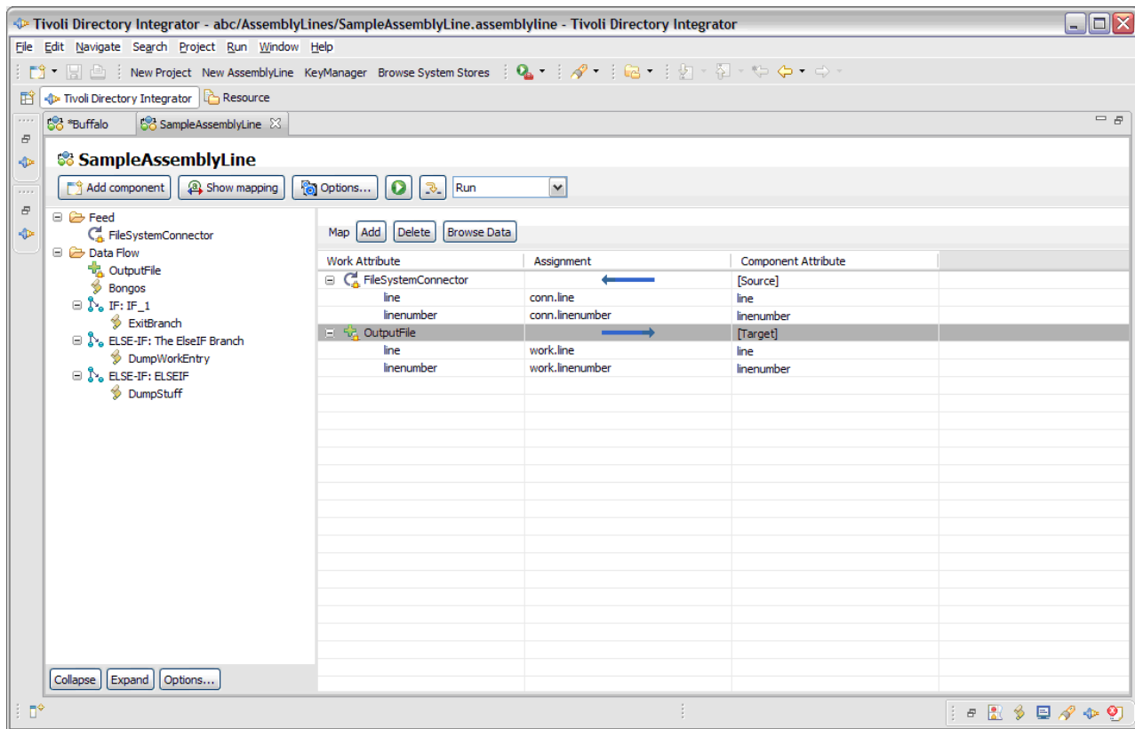
Figure 31. Attribute Mapping
