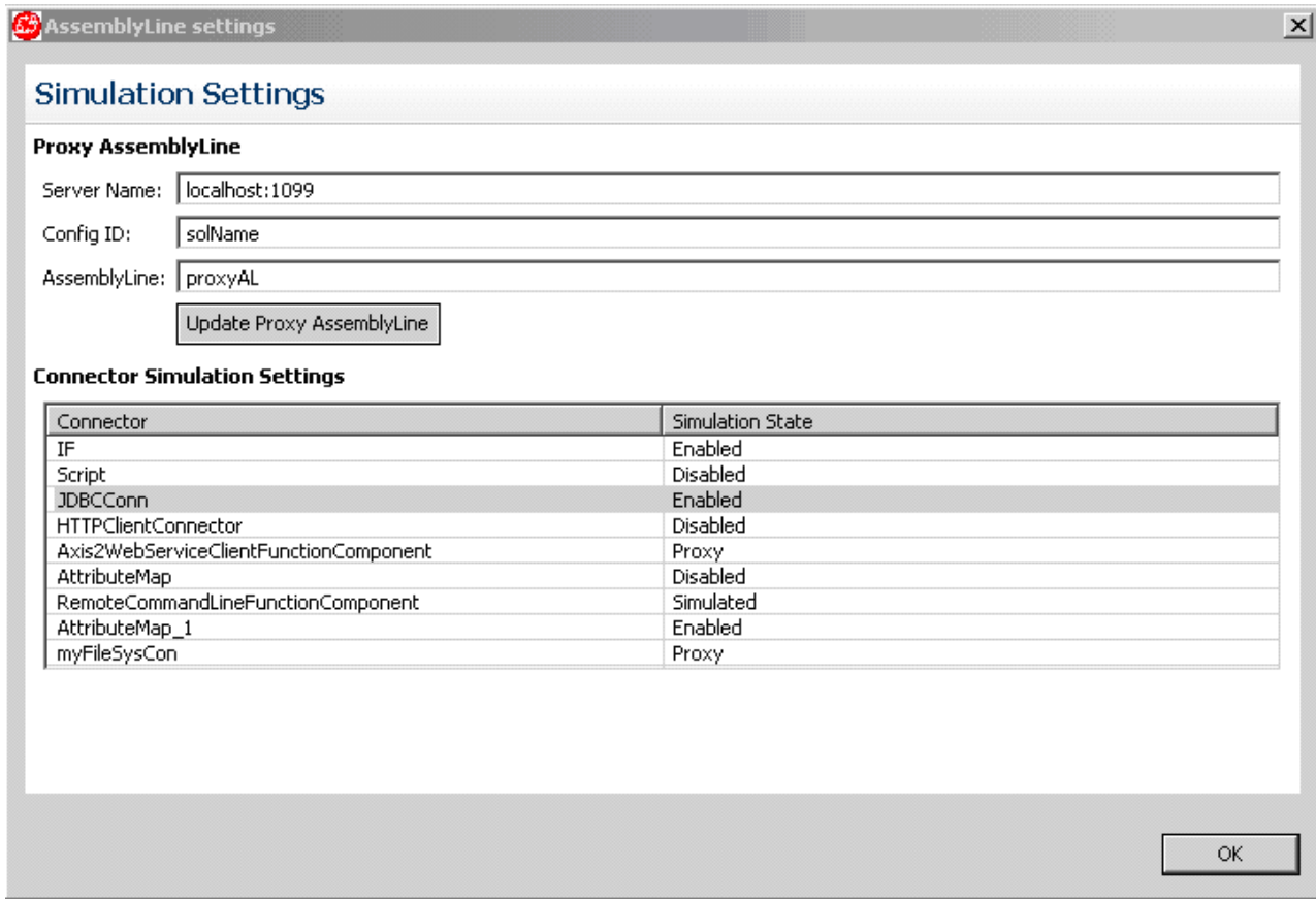
Figure 89. Simulation Settings window
